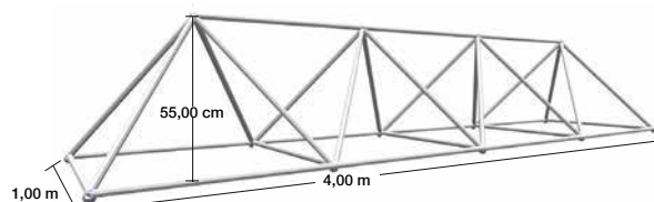
Trellis frame
